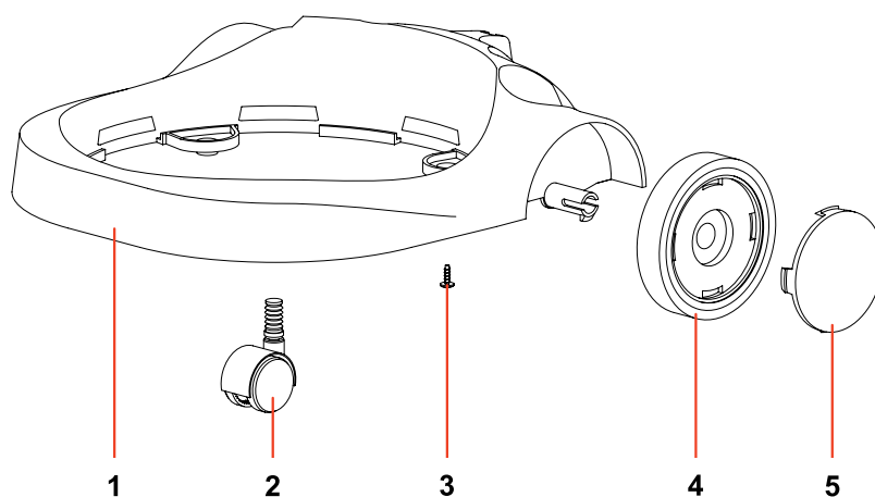
CARRELLO 500 ECO-H FPLAST COMPL. REF. 20884VIA PL
