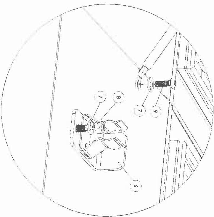
A (1:1)
