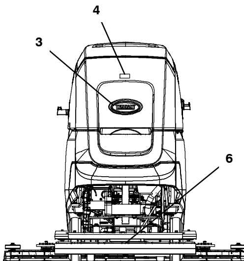
ORBITAL HEAD
